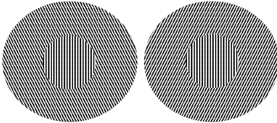
Figure 5: Central circles with vertical lines surrounded by short lines tilted at \pm 20^\circ and \pm 75^\circ respectively.
