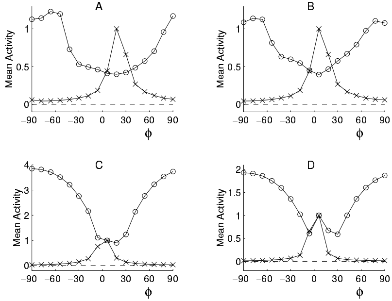
Figure 3: Non-local effects on orientation tuning . (o-o-o) = Center response to preferred orientation at different surround orientations, (x-x-x) = Center orientation tuning without surround stimulation, (-) = Center response to surround stimulation alone. A - response of population with 20° orientation preference. B, C and D - response of populations with 5° orientation preference.
