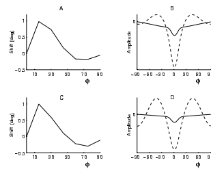
Figure 7: Model simulations of the tilt effect (A and C). B and D show the corresponding kernels mediating long-range interactions. Solid lines indicate the absolute kernel and dashed lines indicate the effective kernel
