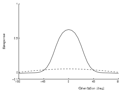
Figure 1: Local tuning curve of horizontal edge detector. Input (--) P = 0.01 \cos(\phi) half width at half height (hw-hh) = 45^\circ , Output (-) hw-hh = 22.5^\circ
