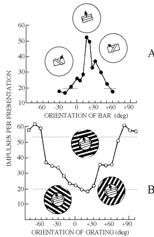
Figure 2: Non-local effects on orientation tuning - experimental data. Response to constant center stimulation at 15^\circ and surround stimulation at angles [-90^\circ, 90^\circ] (open circles), Local tuning curve (filled circles). Redrawn from Blakemore and Tobin (1972)
