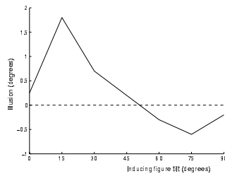
Figure 6: Direct (positive) and indirect (negative) tilt effects
