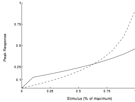
Figure 4: Simulation of weak center stimulus enhancement and strong center stimulus suppression. Center plus surround (-), Center only (- -). Stimulus strength and response normalized to 1
